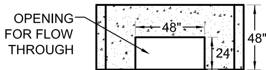
SECTION B-B STIFFENING WALL (IN BASE & EXTENSION SECTIONS)
