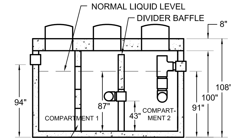
SECTION A-A STIFFENING WALL
